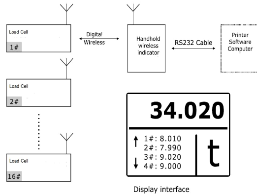
Display interface
